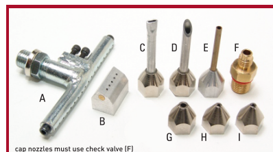
cap nozzles must use check valve (F)
